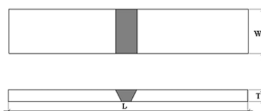
Fig 2. Face bend test specimen top and side views[9]
