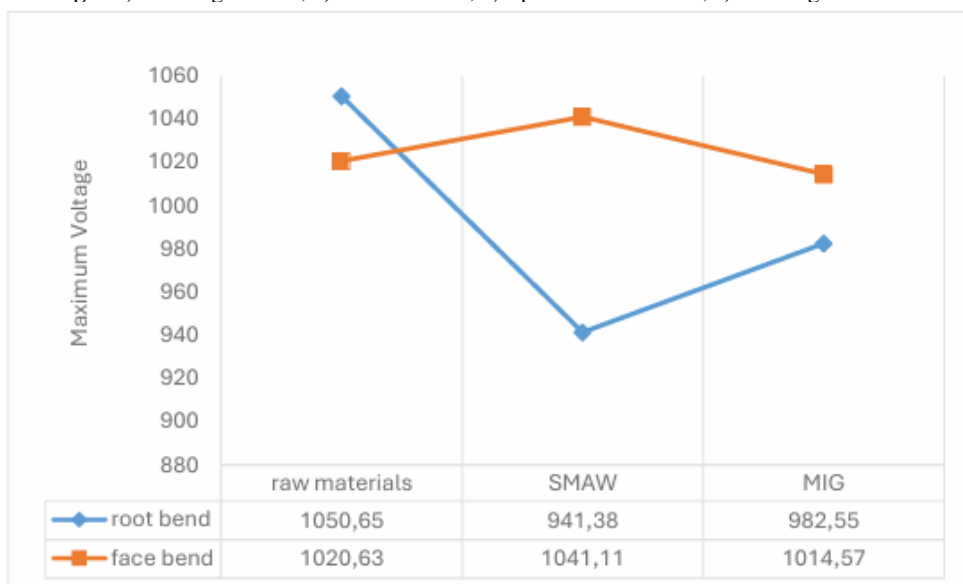
Fig 4. Maximum stress graph of bending test
