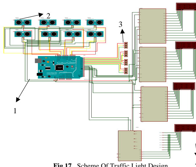
Fig 17. Scheme Of Traffic Light Design
