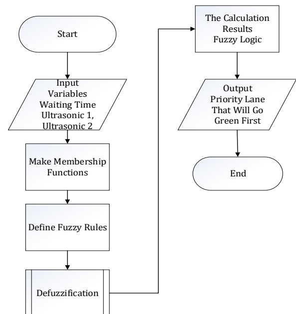
Fig 7. Mamdani Method Flowchart
