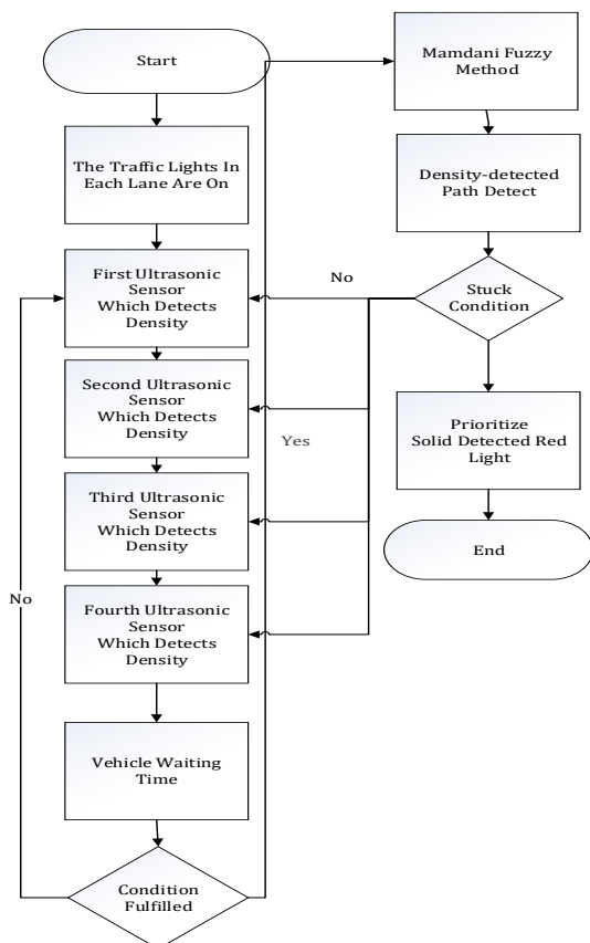
Fig 6. Fuzzy Logic Flowchart
