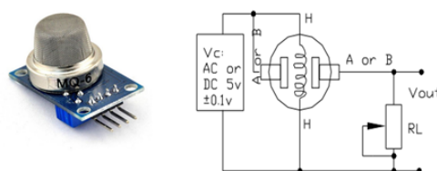
Fig 4. MQ-6 Sensor Module
