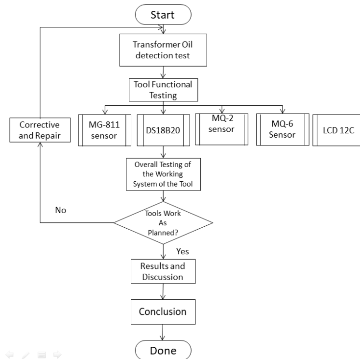
Fig 8. Tool Working Diagram
