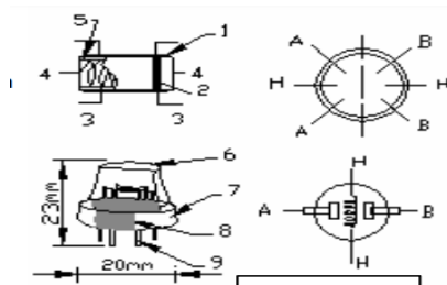
Fig 3. MG-811 Sensor Structure
