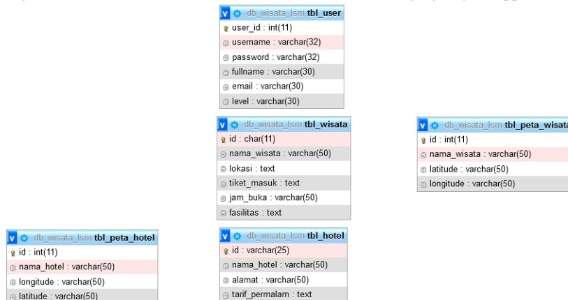
Fig 6. Class Diagram
