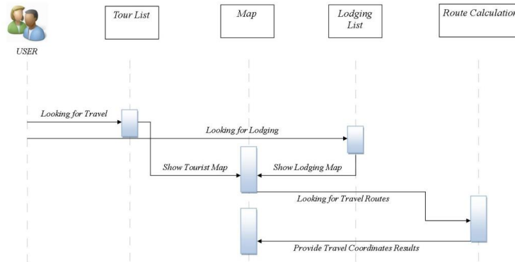
Fig.5 Tourism Object Application Sequence Diagram and Lhokseumawe Lodging Based on Android
