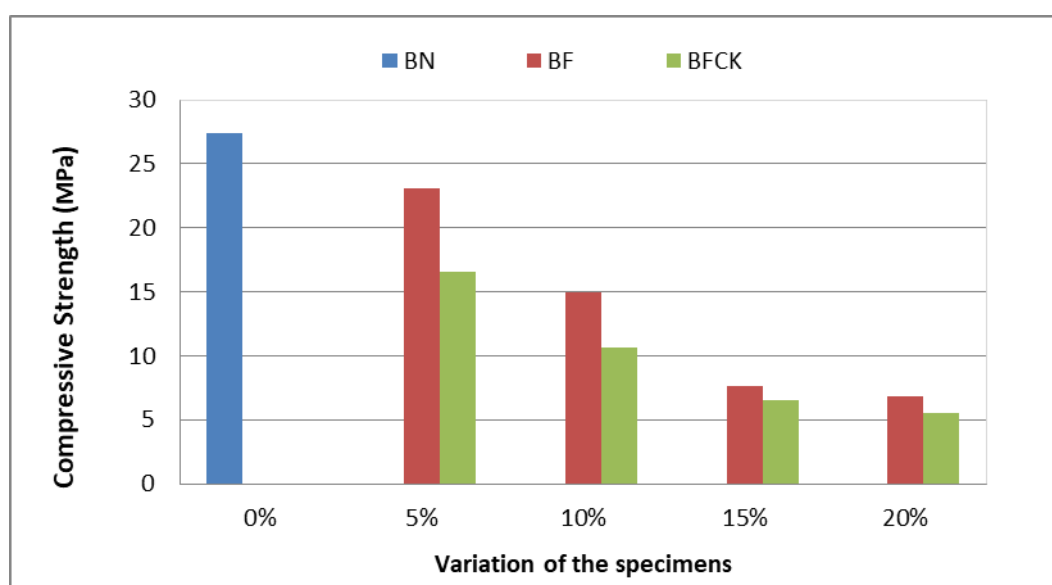
Fig. 2. Compressive strength of concrete
