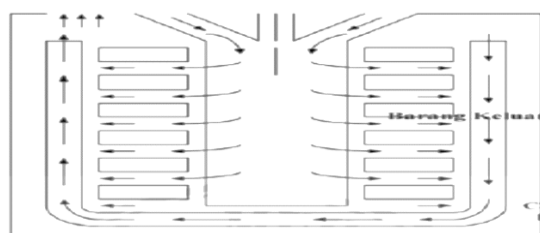
Fig 2: Flow Layout "U"
