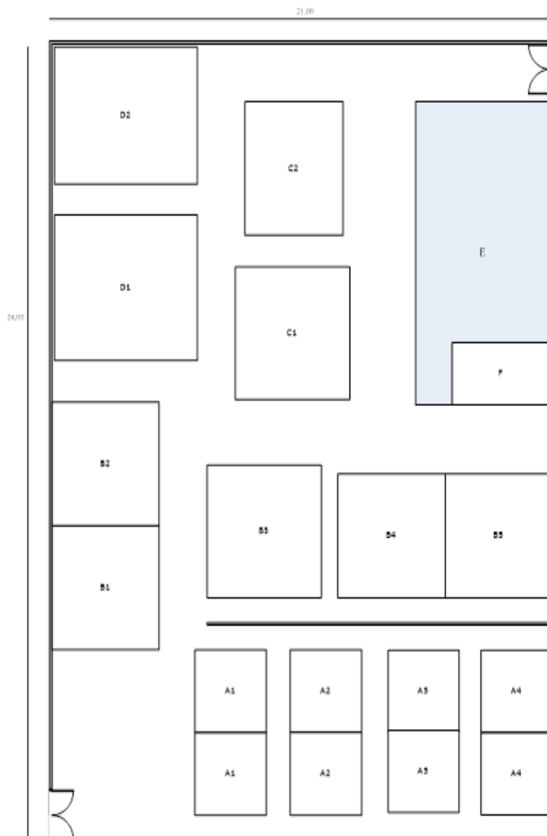
Fig 6: Proposed Warehouse Layout Source: PT. Kilang Padi Mutiara
