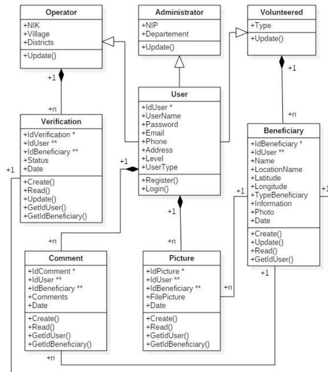
Fig 7. Class diagrams of Infrastructure Model VGI Social Assistance Program
