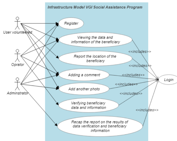
Fig 5. Use Case Diagram of Infrastructure Model VGI Social Assistance Program
